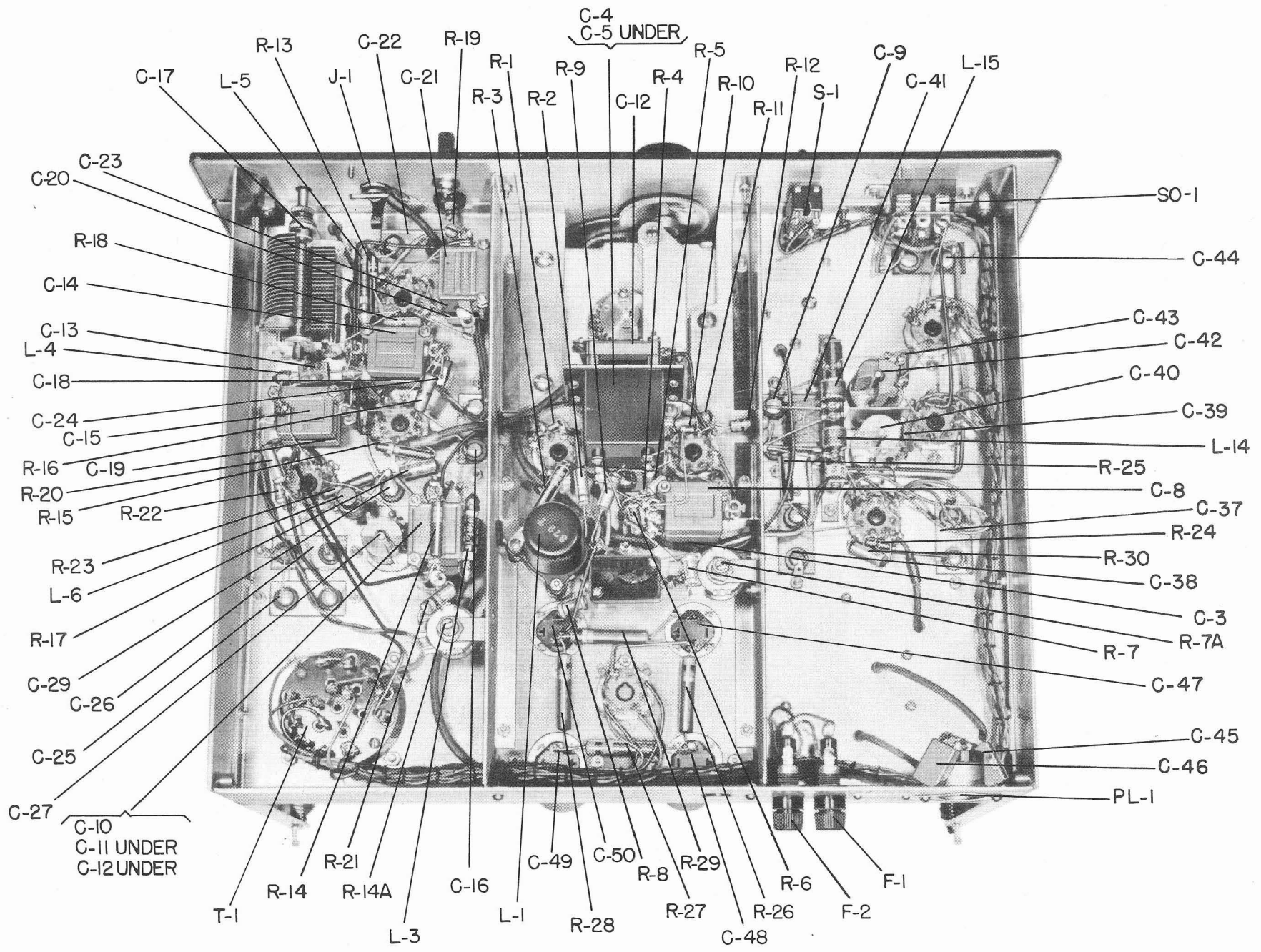
Interior Bottom View of Type 1110-A Interpolating Frequency Standard
