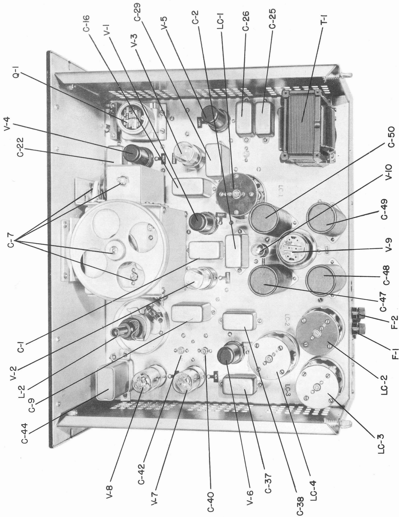
Interior Top View of Type 1110-A Interpolating Frequency Standard
