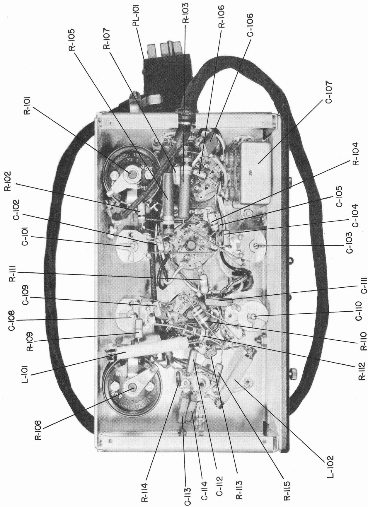
Interior Bottom View of Type 1110-P1 Multivibrator
